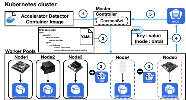
Figure 2: The implementation of accelerator hardware information extraction module
